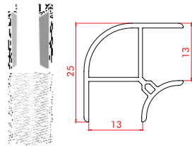
UNS-81545.10/12/15 90° Baza Köşe UNS-81545.10/12/15 90° Plinth Corner
