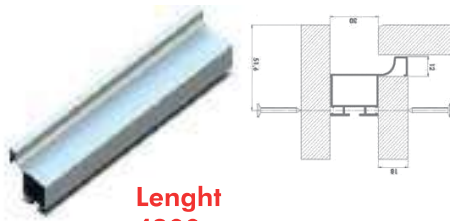
UNS-81523 Gola Diley L Profili UNS-81523 Gola Vertical L Profile
