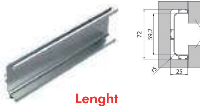
UNS-81522 Gola Yatay U Profili UNS-81522 Gola Horizontal U Profile
