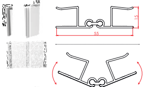
UNS-81544.10/12/15 Ayarlı Baza Köşe UNS-81544.10/12/15 Adjustable PVC Plinth Corner
