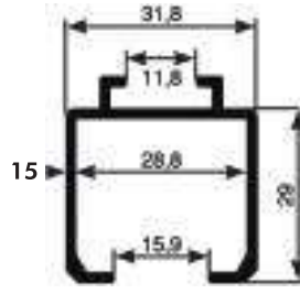
91023 Alt ve Üst Ray 91023 Down and Up Rail
