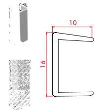
UNS-81547.10/12/15 Baza Köşe Kapama UNS-81547.10/12/15 PVC Plinth End Cap
