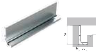
UNS-81521 Gola Yatay L Profili UNS-81521 Gola Horizontal L Profile
