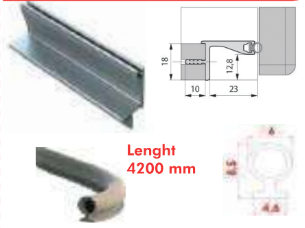
UNS-81525 Gola Fitilli Üst Profili UNS-81525 Gola Upper Profile With Rubber
