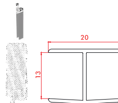
UNS-81546.10/12/15 Baza Ara Birleştirici UNS-81546.10/12/15 PVC Plinth Joint
